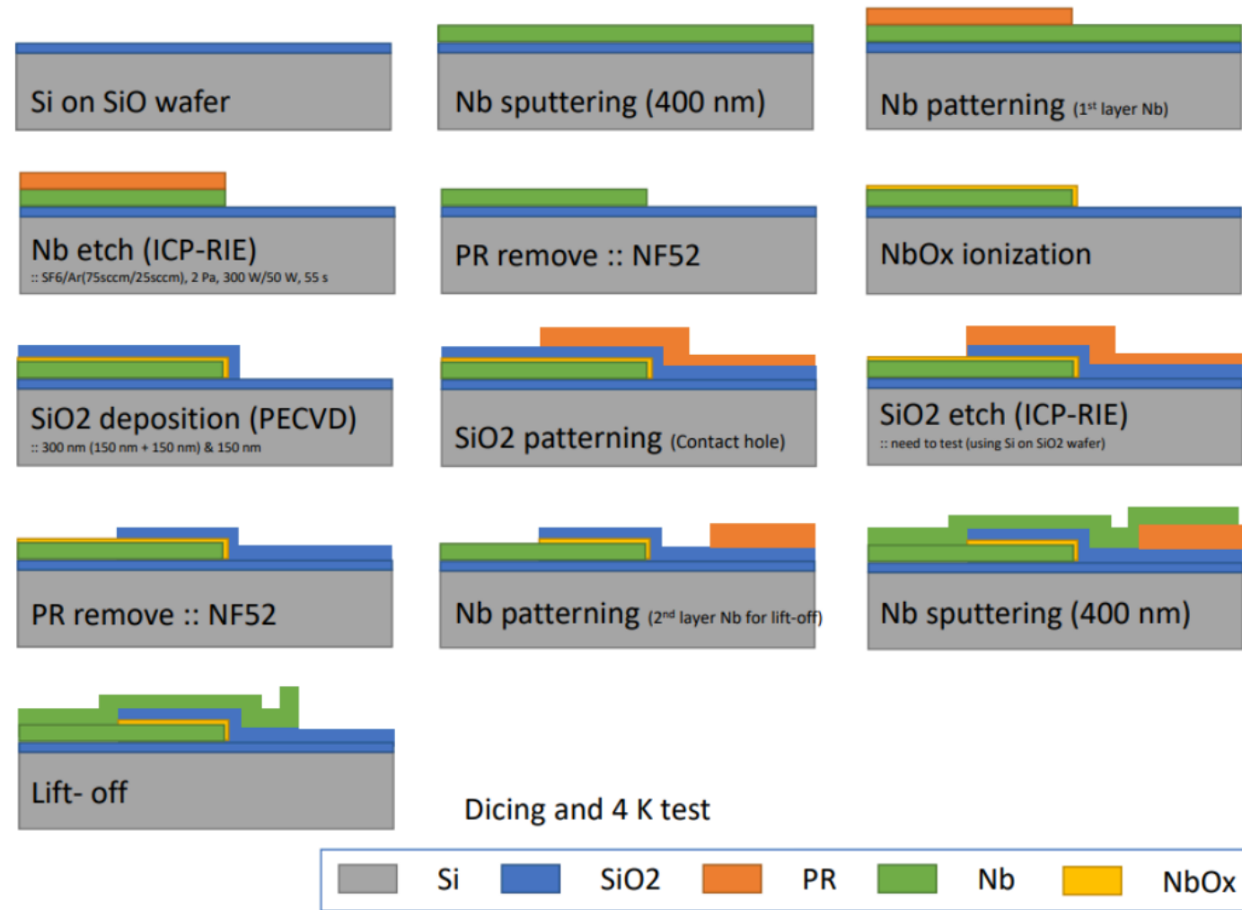
Nb 2layer Fabrication process for contact test
