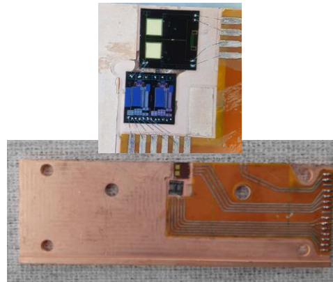
Sensor chip attachment
