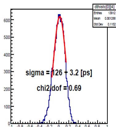
Linear inverse interpolation
