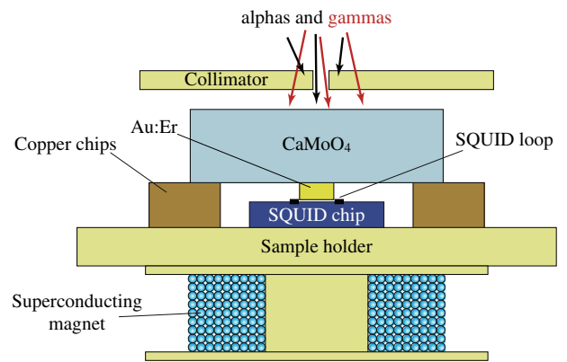
Fig. 1. A schematic diagram of the detector setup (not to scale). Alphas and gammas from an ^{241}\text{Am} source are absorbed in a \text{CaMoO}_4 crystal. The resulting increase in temperature is measured by an MMC with a Au:Er sensor positioned in the pick-up loop of a dc-SQUID. A superconducting magnet is used to magnetize the Au:Er sensor.
