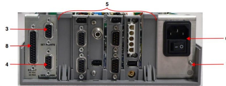
Figure 1-2 Backplate Connections (CNV, IMG, Analog and HFIG boards shown)
