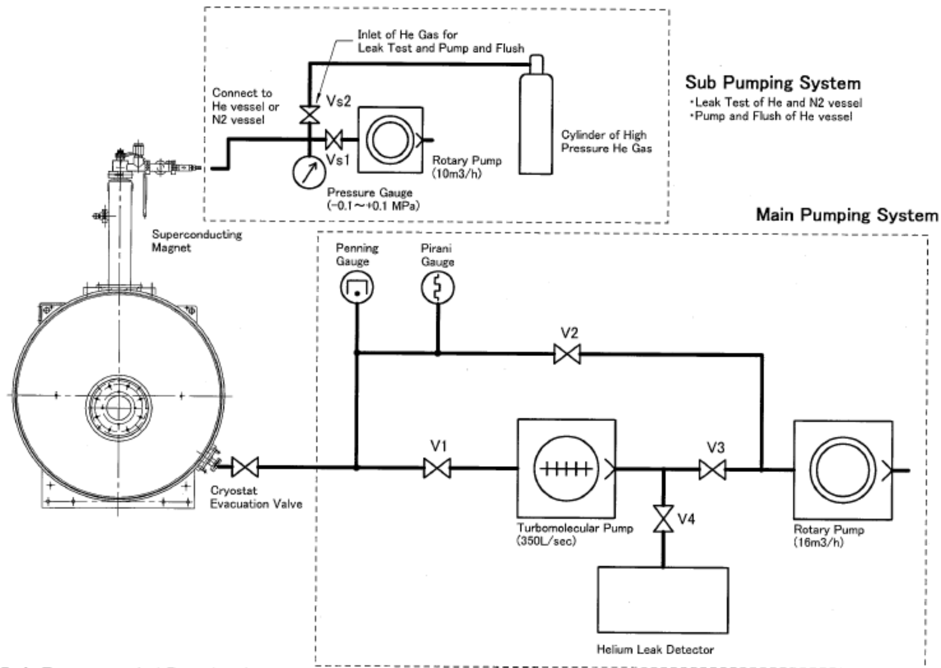
Figure 5-4 Recommended Pumping System
